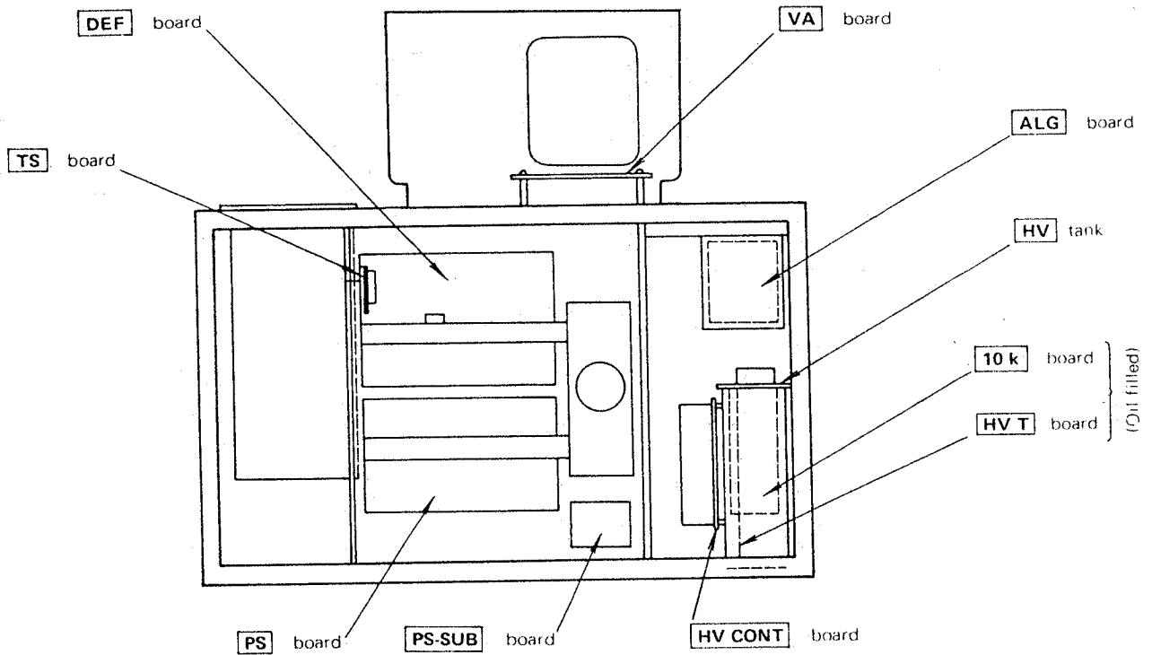
Rear View
